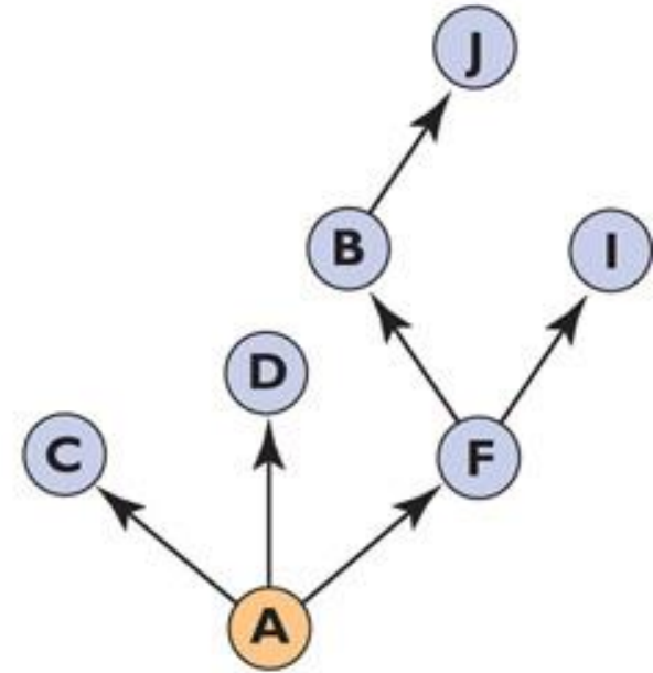
Cluster
