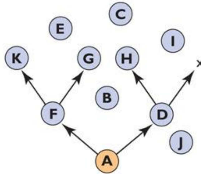
Probability
